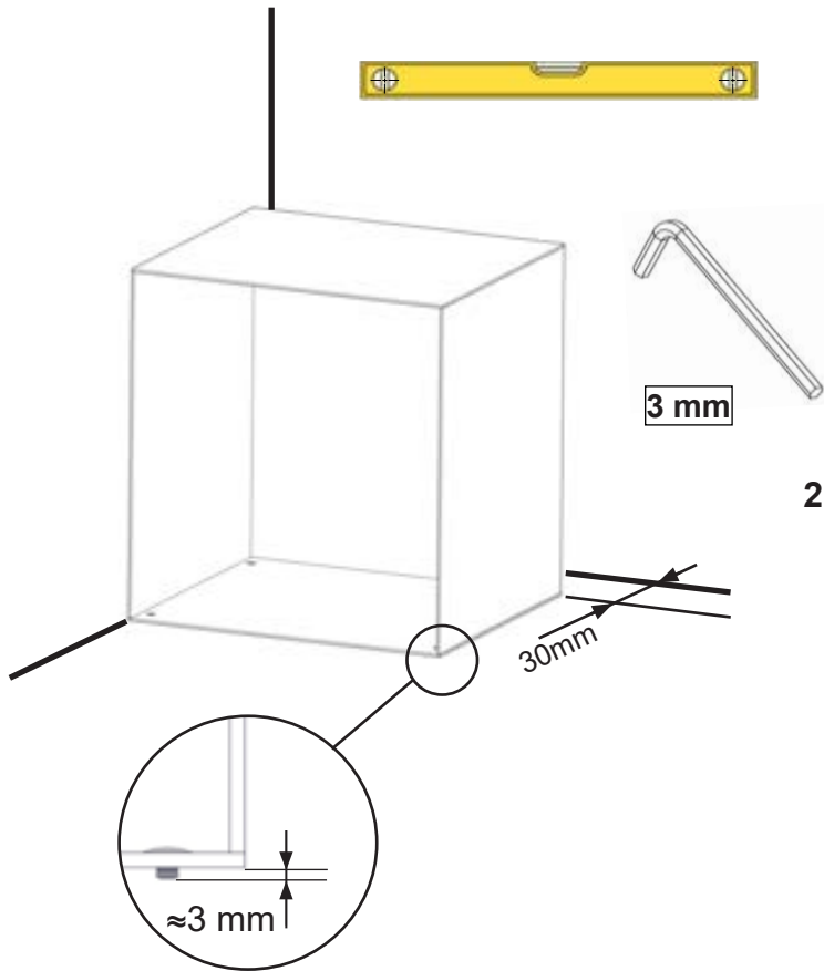
Module large / small
